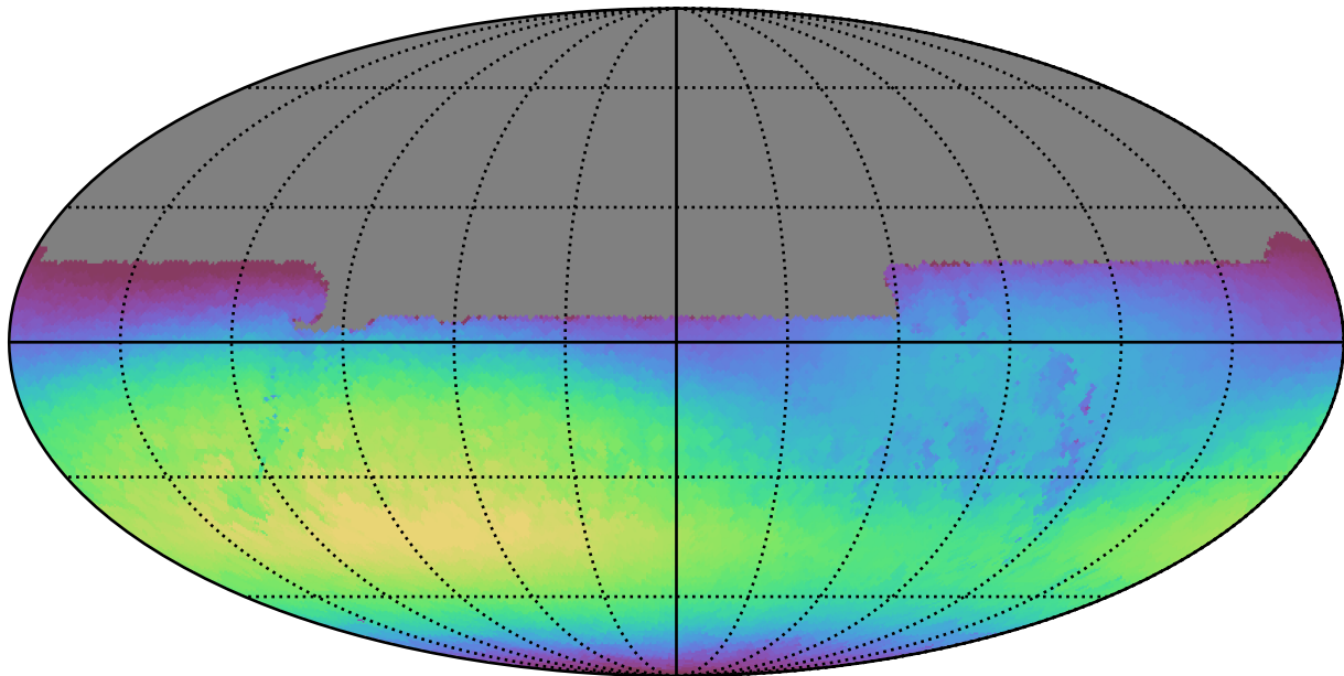
mw_roll_all_v3.3_10yrs All sky u band: Max skyBrightness
