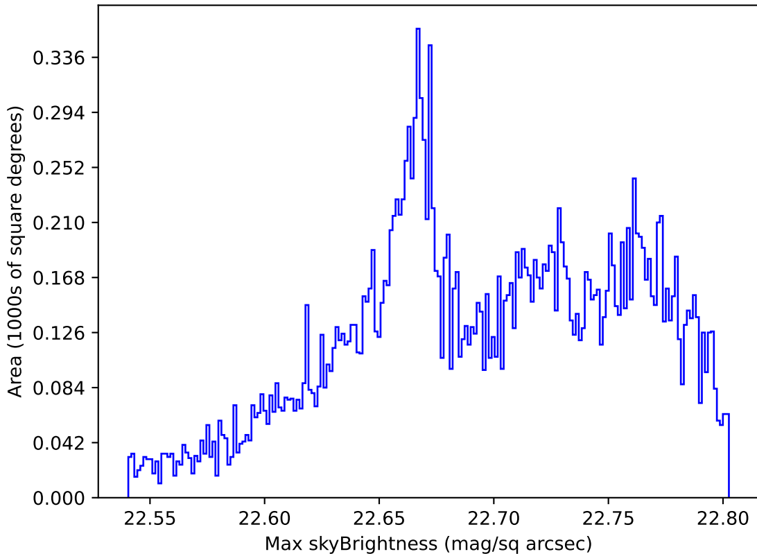
mw_roll_all_v3.3_10yrs All sky u band: Max skyBrightness
