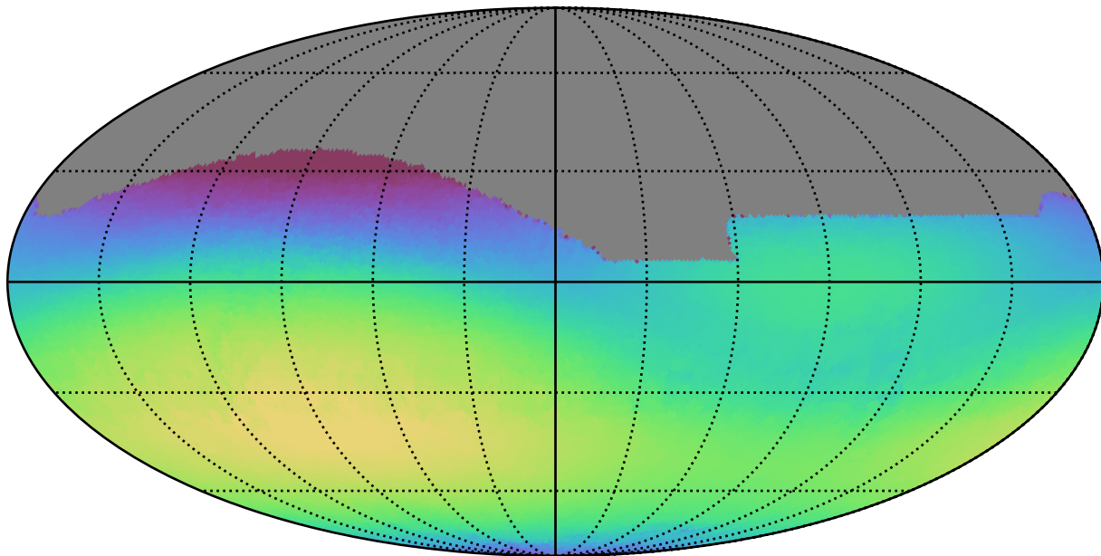
mw_roll_all_v3.3_10yrs All sky r band: Max skyBrightness
