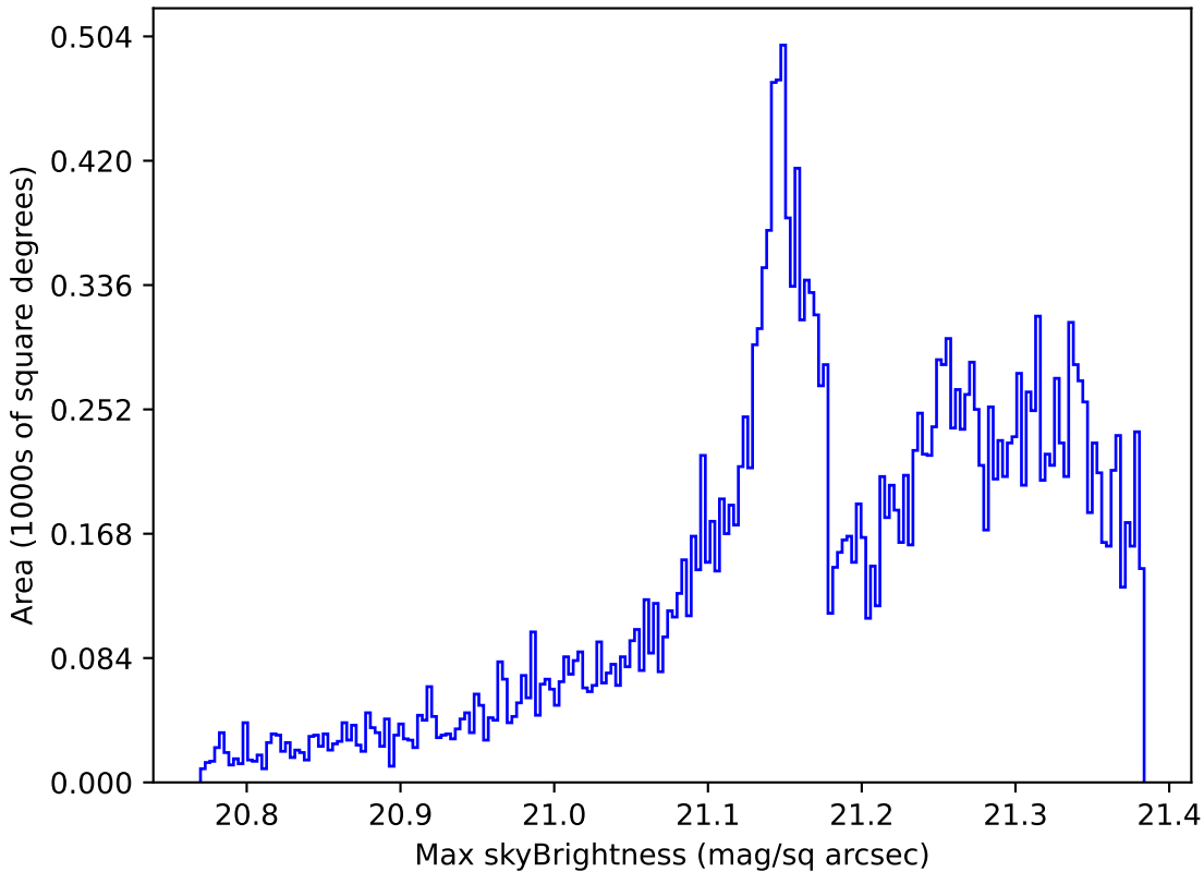
mw_roll_all_v3.3_10yrs All sky r band: Max skyBrightness
