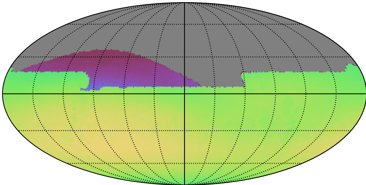
mw_roll_all_v3.3_10yrs All sky all bands: Max skyBrightness
