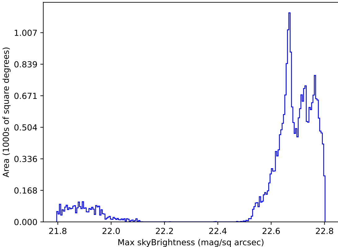
mw_roll_all_v3.3_10yrs All sky all bands: Max skyBrightness
