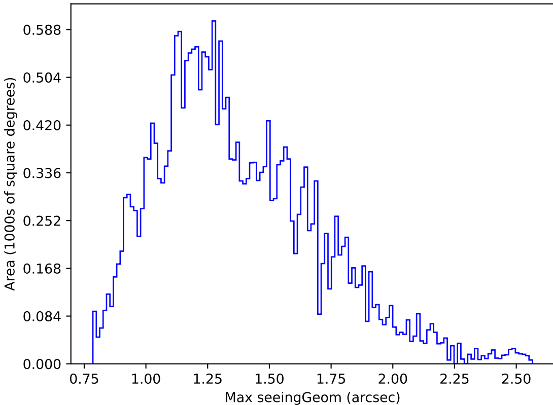
mw_roll_all_v3.3_10yrs Yr 1 r band: Max seeingGeom
