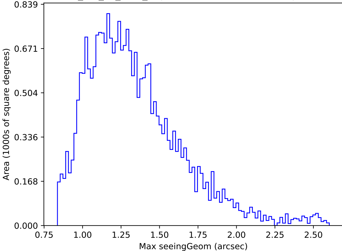
mw_roll_all_v3.3_10yrs Yr 1 i band: Max seeingGeom
