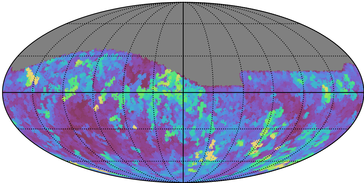
mw_roll_all_v3.3_10yrs Yr 1 all bands: Max seeingGeom
