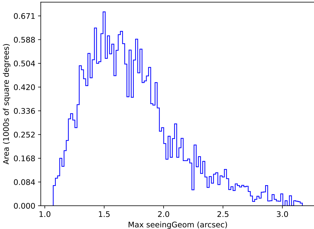
mw_roll_all_v3.3_10yrs Yr 1 all bands: Max seeingGeom
