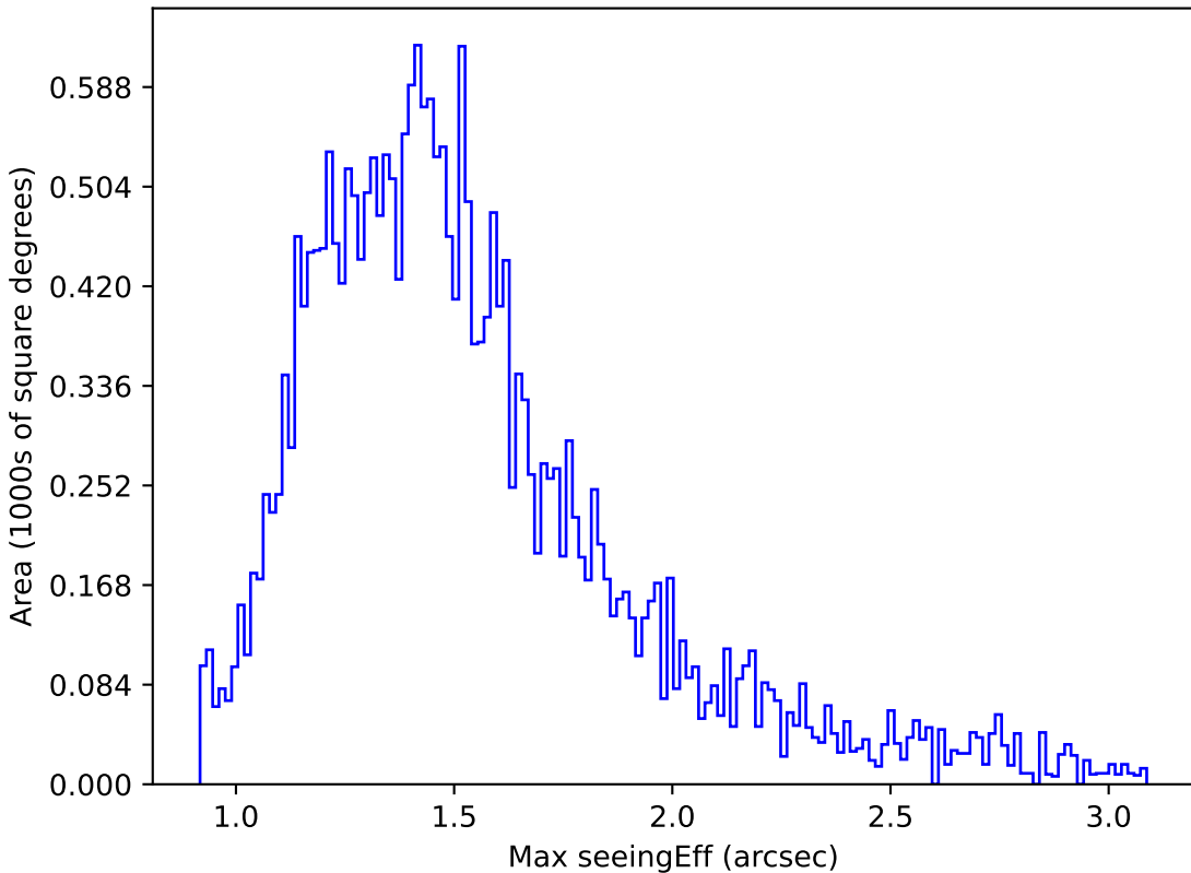
mw_roll_all_v3.3_10yrs Yr 1 z band: Max seeingEff
