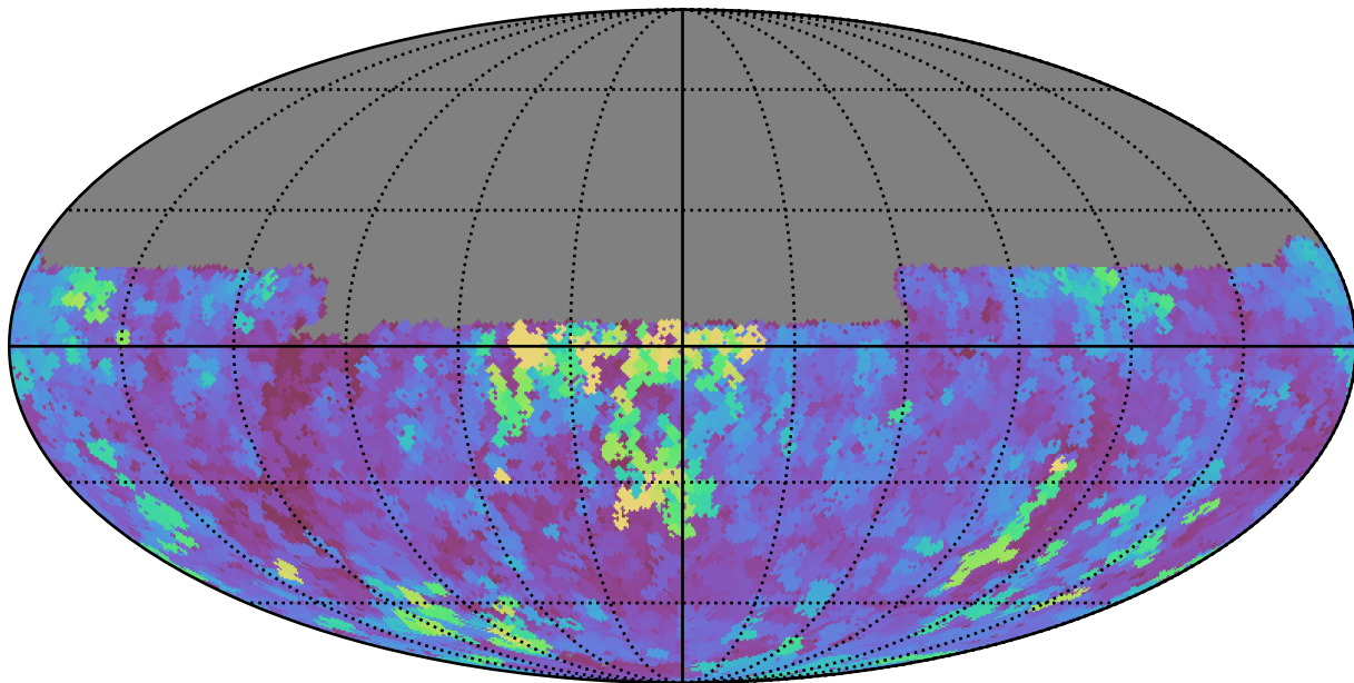
mw_roll_all_v3.3_10yrs Yr 1 y band: Max seeingEff
