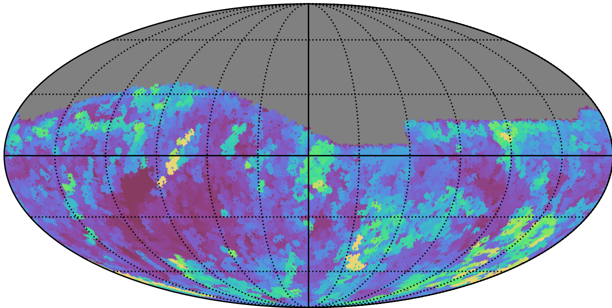
mw_roll_all_v3.3_10yrs Yr 1 r band: Max seeingEff
