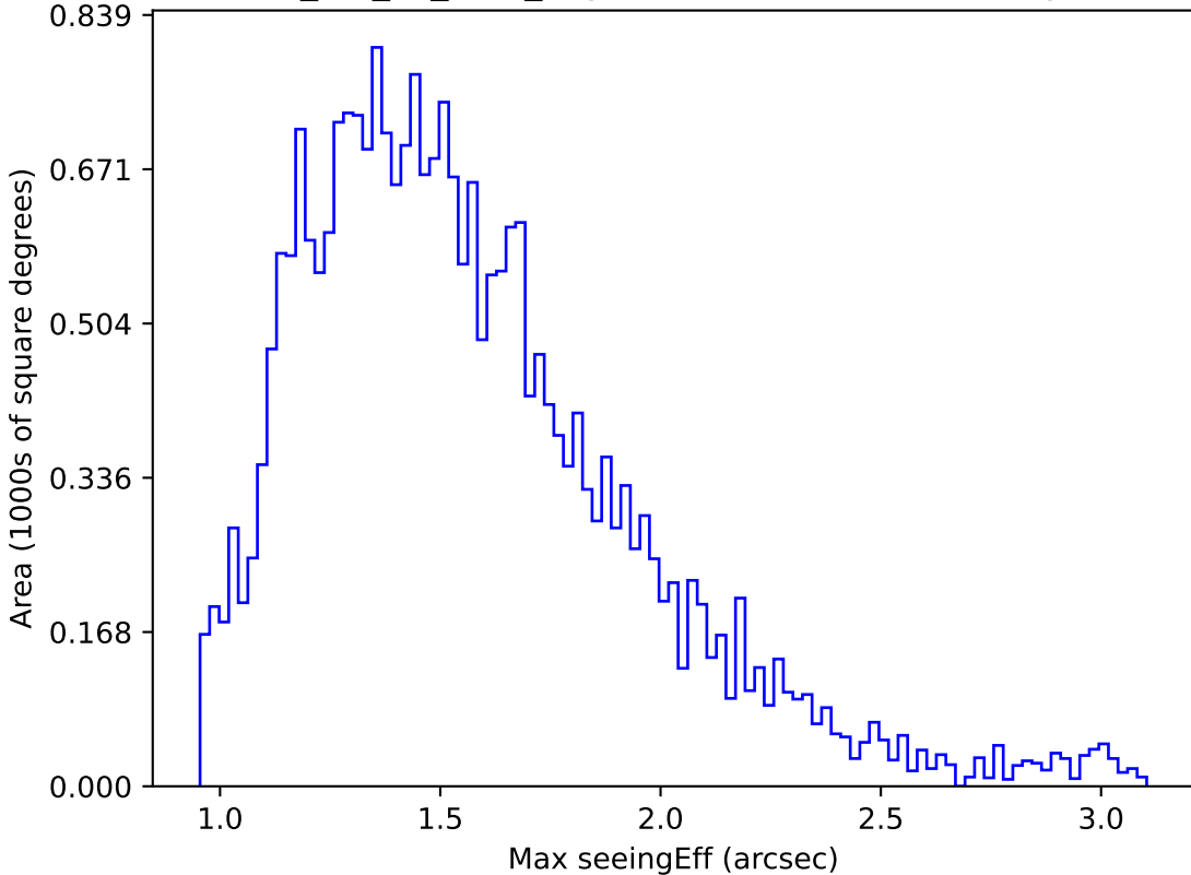
mw_roll_all_v3.3_10yrs Yr 1 i band: Max seeingEff
