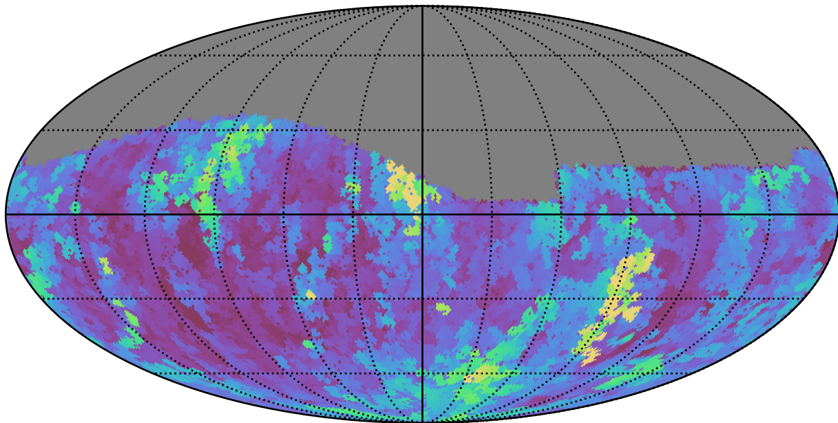
mw_roll_all_v3.3_10yrs Yr 1 g band: Max seeingEff
