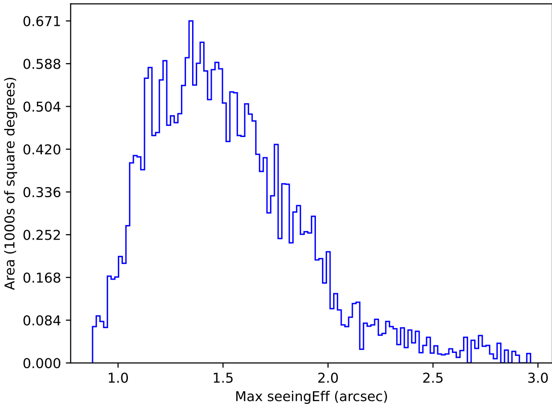
mw_roll_all_v3.3_10yrs Yr 1 g band: Max seeingEff
