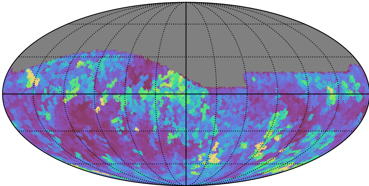
mw_roll_all_v3.3_10yrs Yr 1 all bands: Max seeingEff
