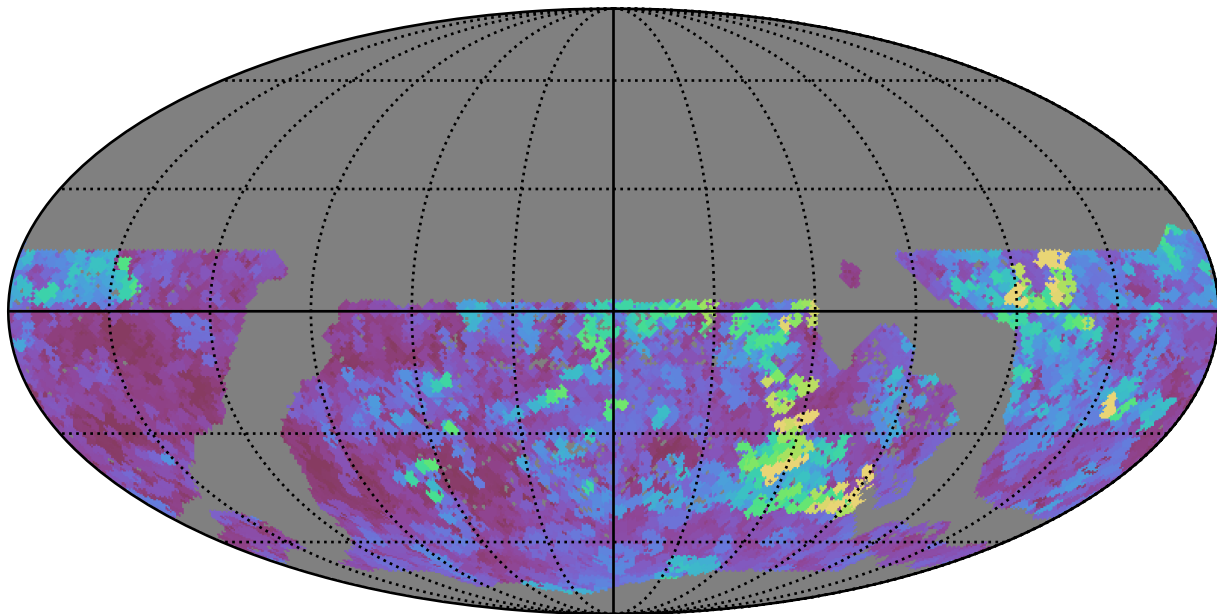
mw_roll_all_v3.3_10yrs WFD y band: Max seeingEff
