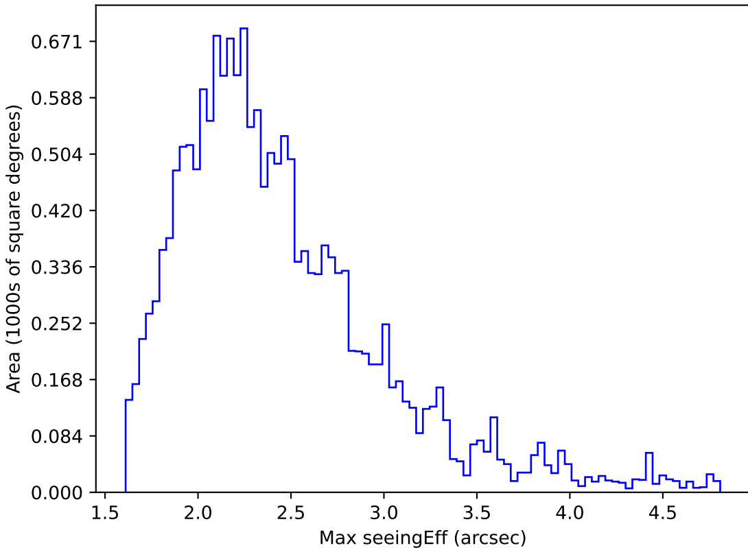
mw_roll_all_v3.3_10yrs WFD y band: Max seeingEff
