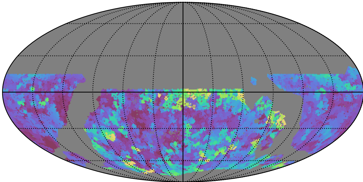
mw_roll_all_v3.3_10yrs WFD u band: Max seeingEff
