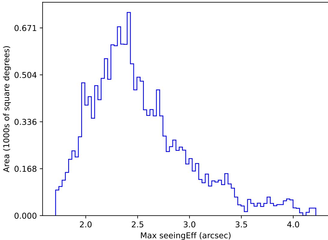
mw_roll_all_v3.3_10yrs WFD u band: Max seeingEff
