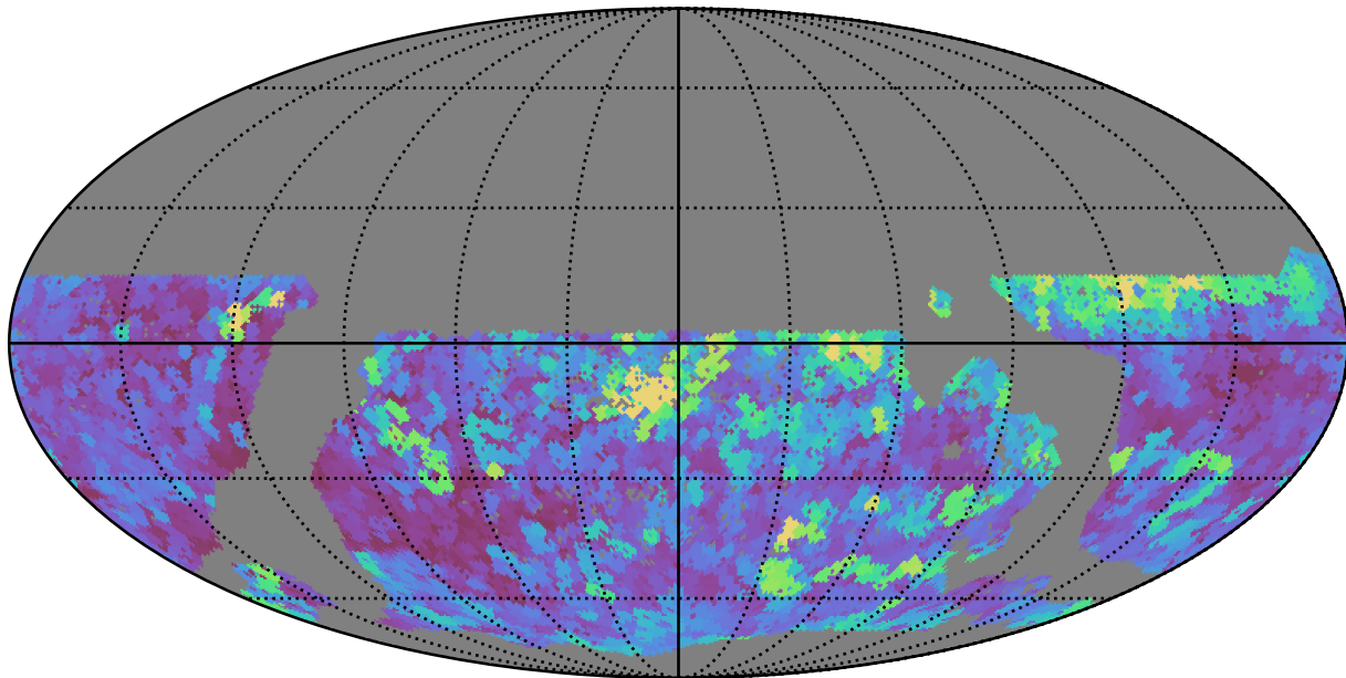
mw_roll_all_v3.3_10yrs WFD r band: Max seeingEff
