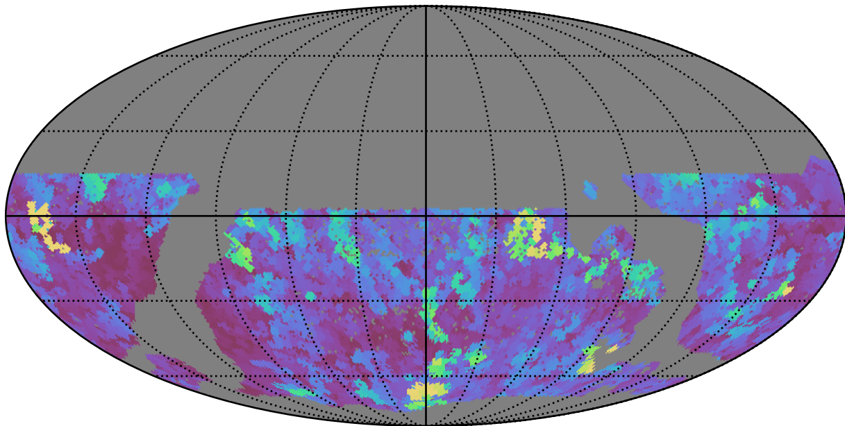
mw_roll_all_v3.3_10yrs WFD i band: Max seeingEff
