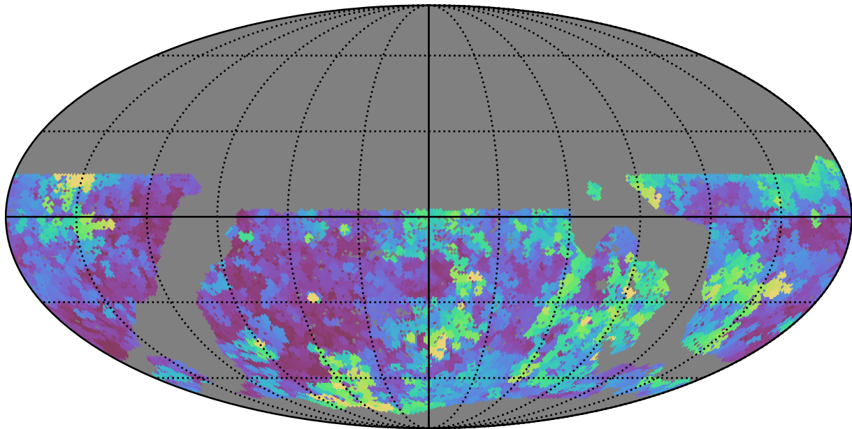
mw_roll_all_v3.3_10yrs WFD g band: Max seeingEff
