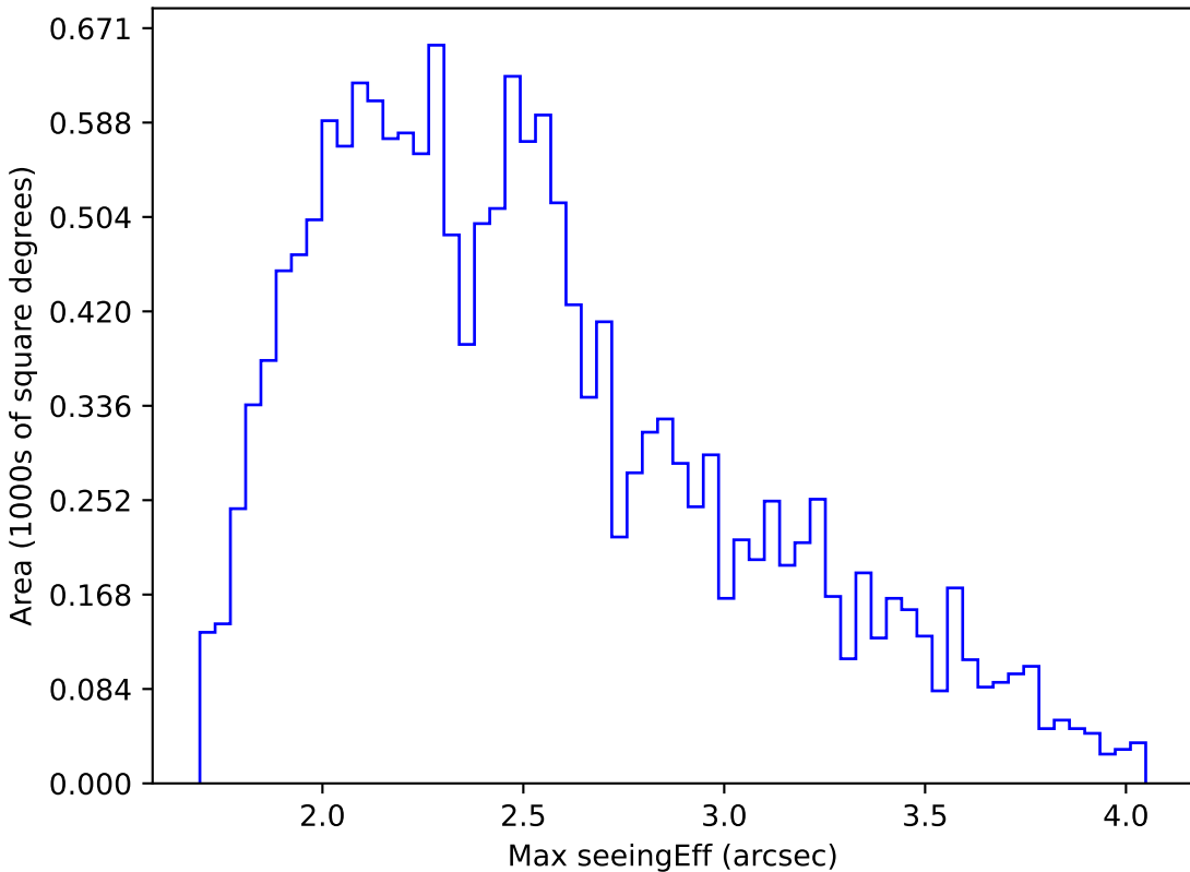
mw_roll_all_v3.3_10yrs WFD g band: Max seeingEff
