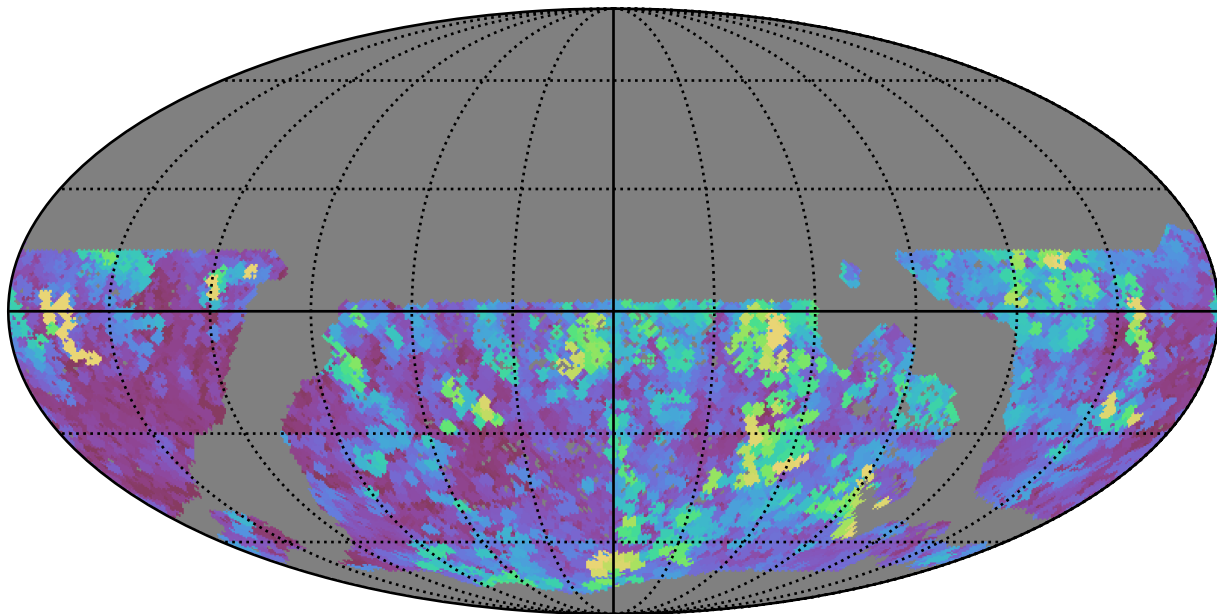
mw_roll_all_v3.3_10yrs WFD all bands: Max seeingEff
