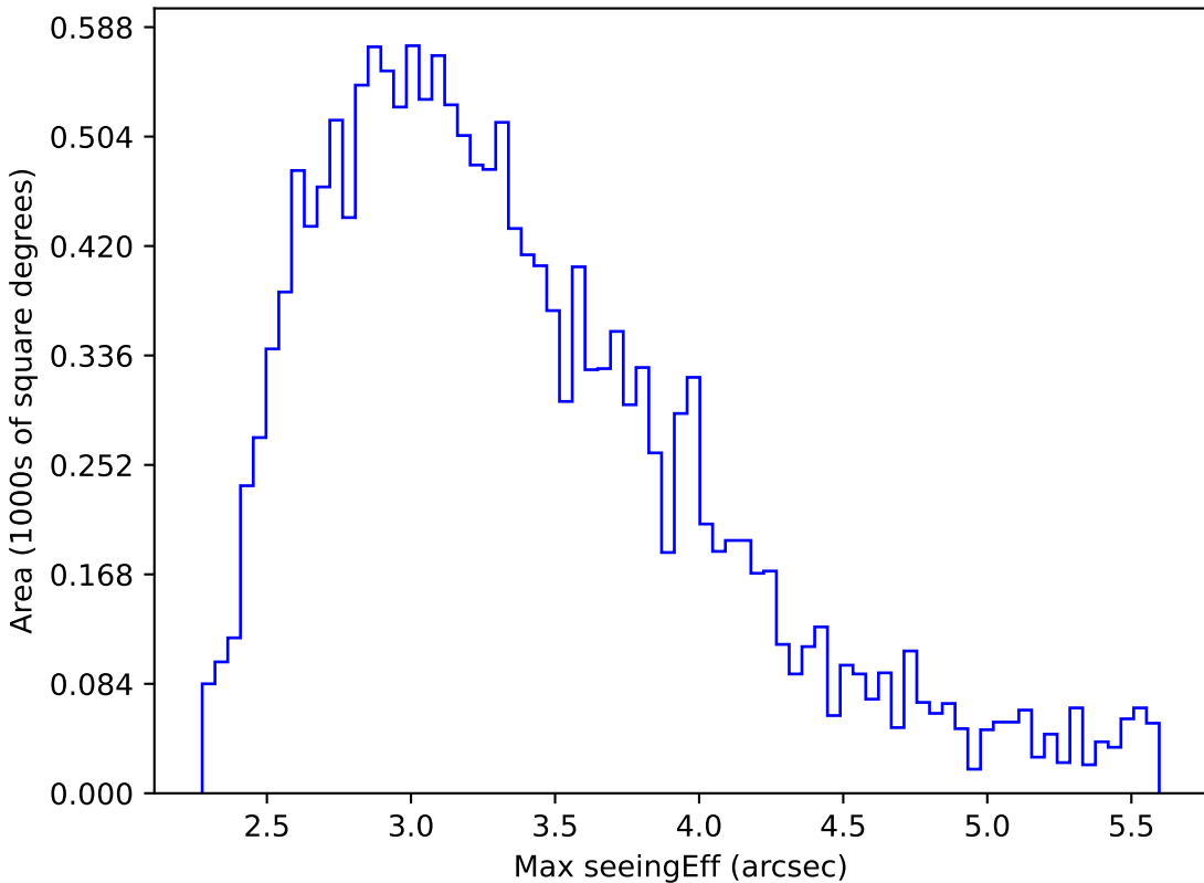
mw_roll_all_v3.3_10yrs WFD all bands: Max seeingEff
