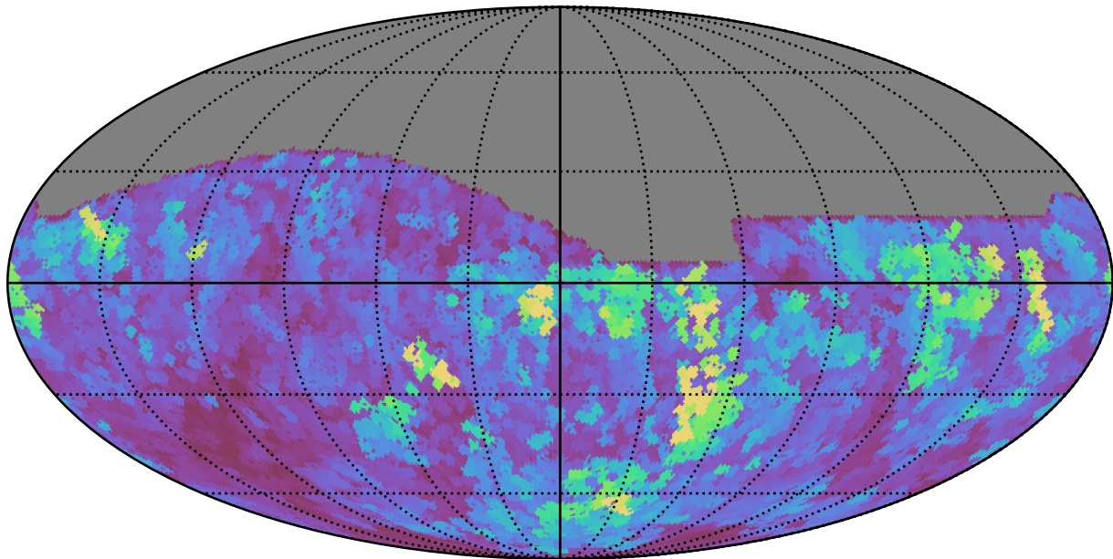
mw_roll_all_v3.3_10yrs All sky z band: Max seeingEff
