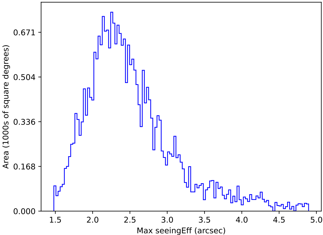
mw_roll_all_v3.3_10yrs All sky z band: Max seeingEff
