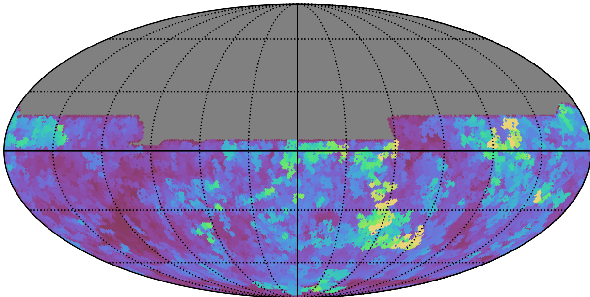
mw_roll_all_v3.3_10yrs All sky y band: Max seeingEff
