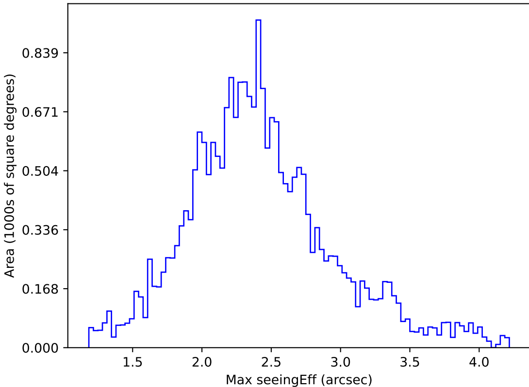
mw_roll_all_v3.3_10yrs All sky u band: Max seeingEff
