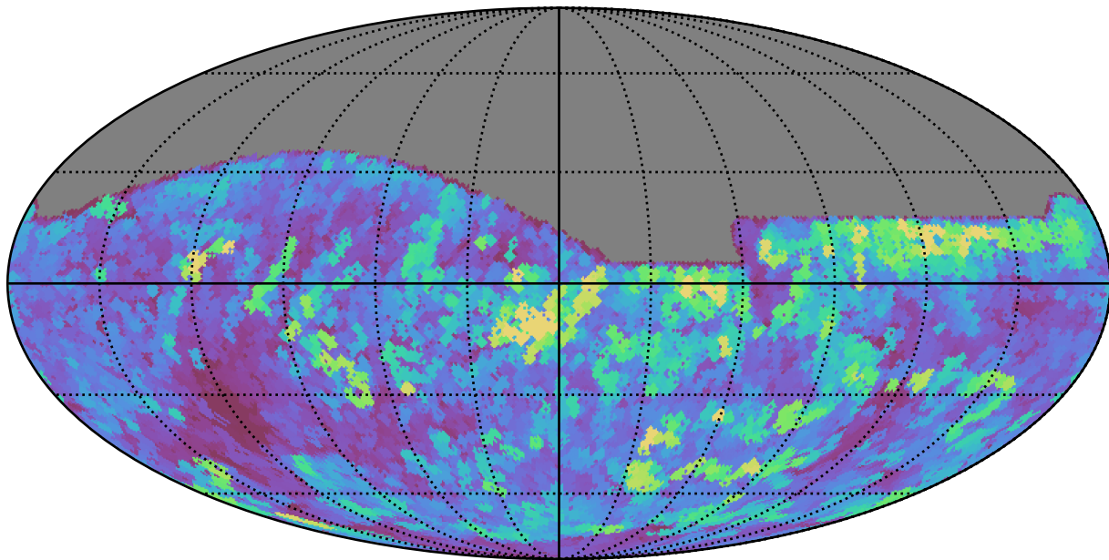
mw_roll_all_v3.3_10yrs All sky r band: Max seeingEff
