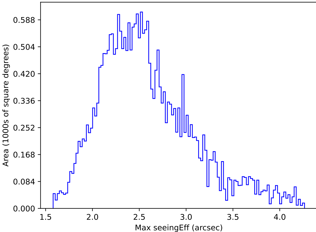
mw_roll_all_v3.3_10yrs All sky r band: Max seeingEff
