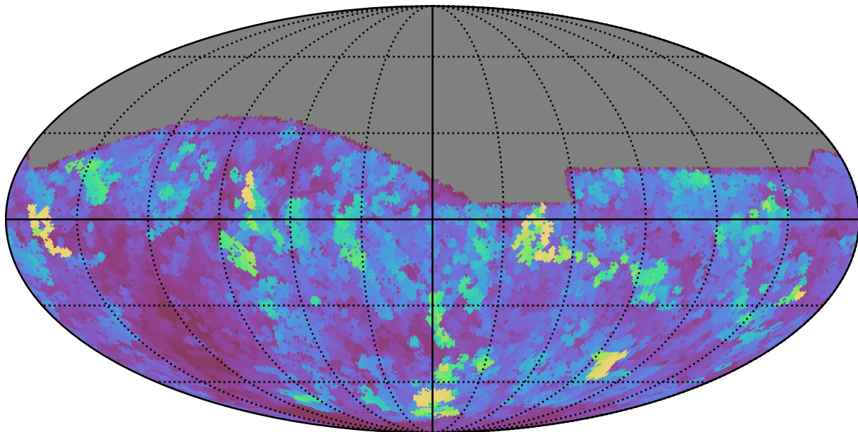
mw_roll_all_v3.3_10yrs All sky i band: Max seeingEff
