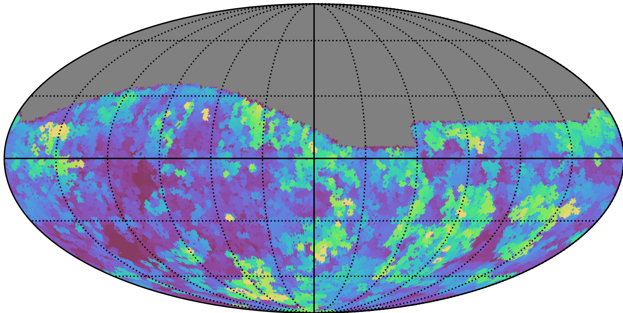
mw_roll_all_v3.3_10yrs All sky g band: Max seeingEff
