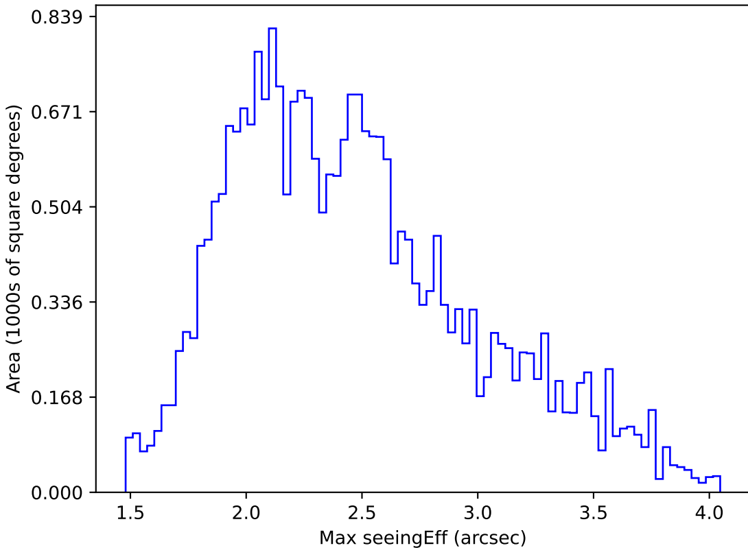
mw_roll_all_v3.3_10yrs All sky g band: Max seeingEff
