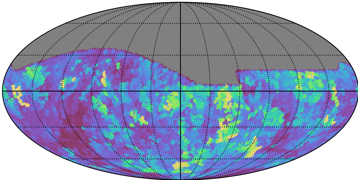
mw_roll_all_v3.3_10yrs All sky all bands: Max seeingEff
