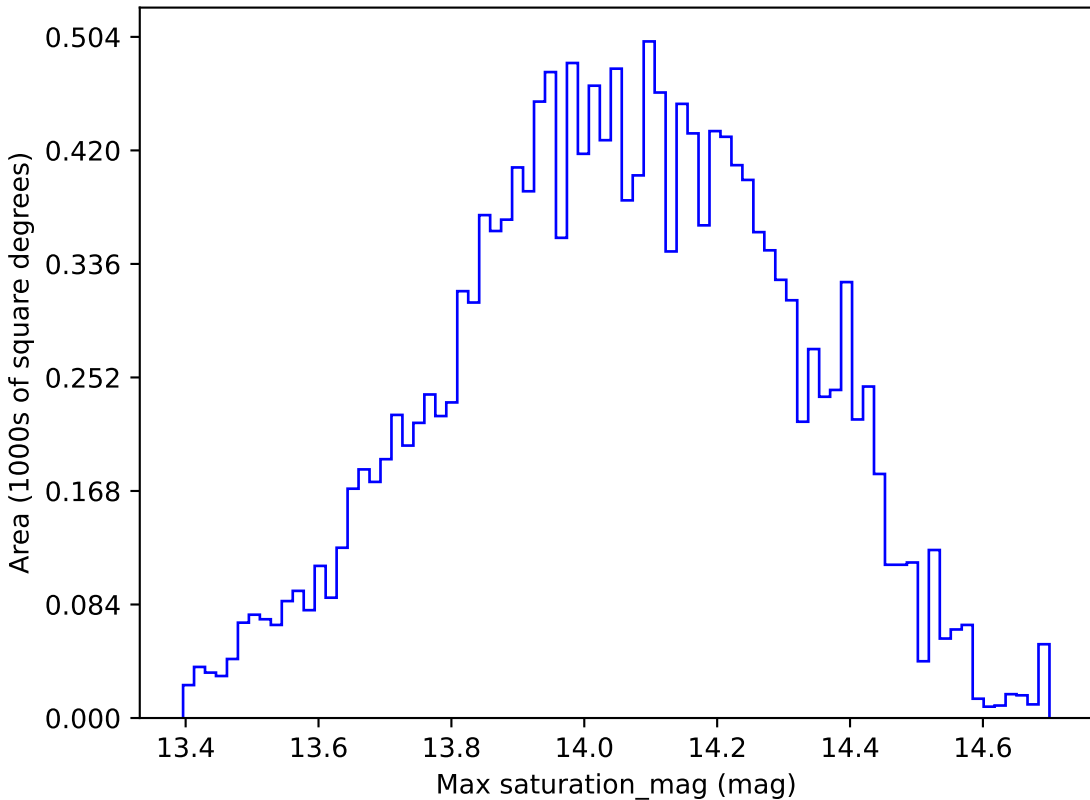
mw_roll_all_v3.3_10yrs WFD u band: Max saturation_mag
