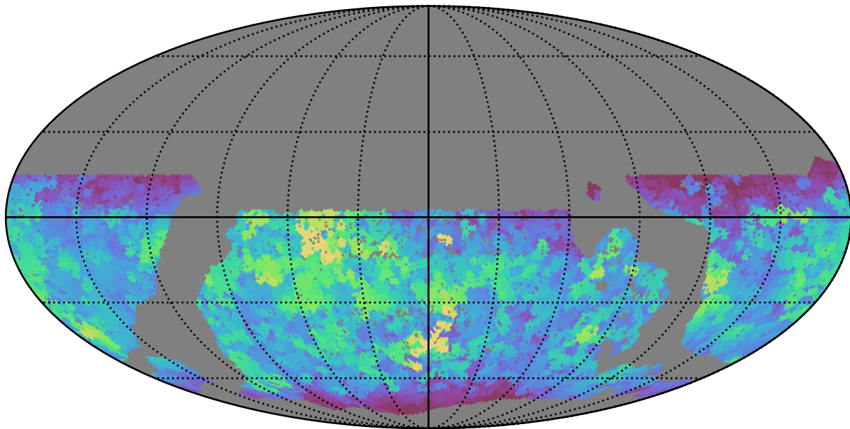
mw_roll_all_v3.3_10yrs WFD all bands: Max saturation_mag
