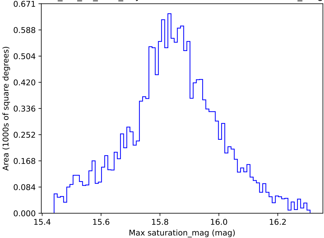
mw_roll_all_v3.3_10yrs WFD all bands: Max saturation_mag
