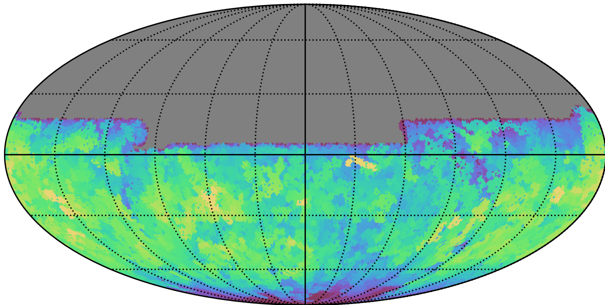
mw_roll_all_v3.3_10yrs All sky u band: Max saturation_mag
