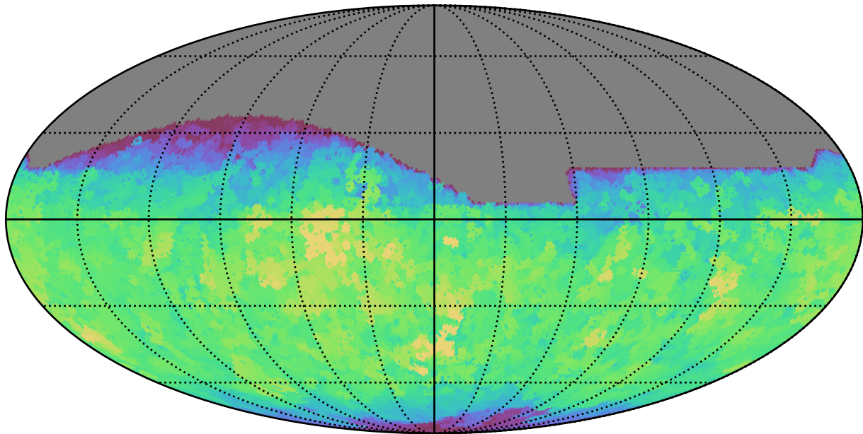
mw_roll_all_v3.3_10yrs All sky all bands: Max saturation_mag
