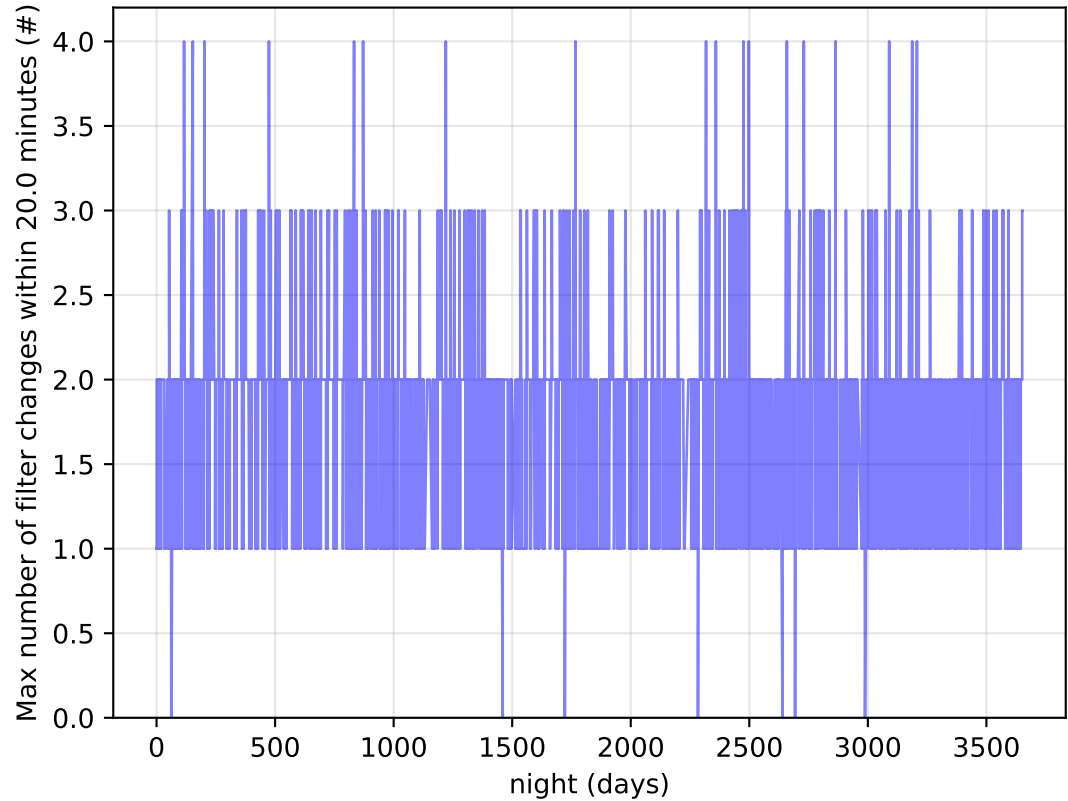
mw_roll_all_v3.3_10yrs Per Night: Max number of filter changes within 20.0 minutes
