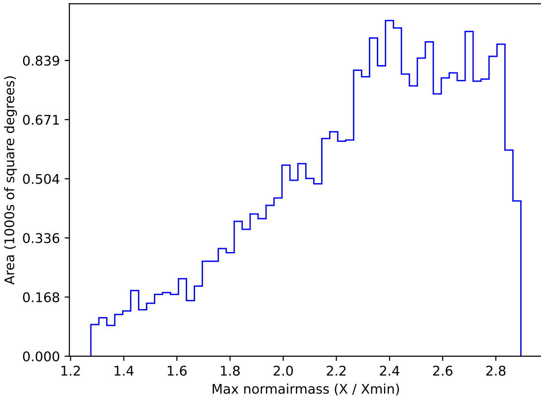
mw_roll_all_v3.3_10yrs All sky all bands: Max normairmass
