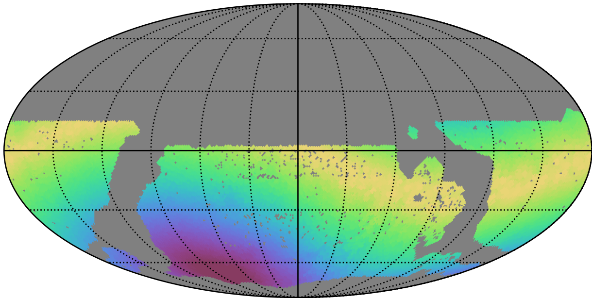
mw_roll_all_v3.3_10yrs WFD r band: Max moonDistance
