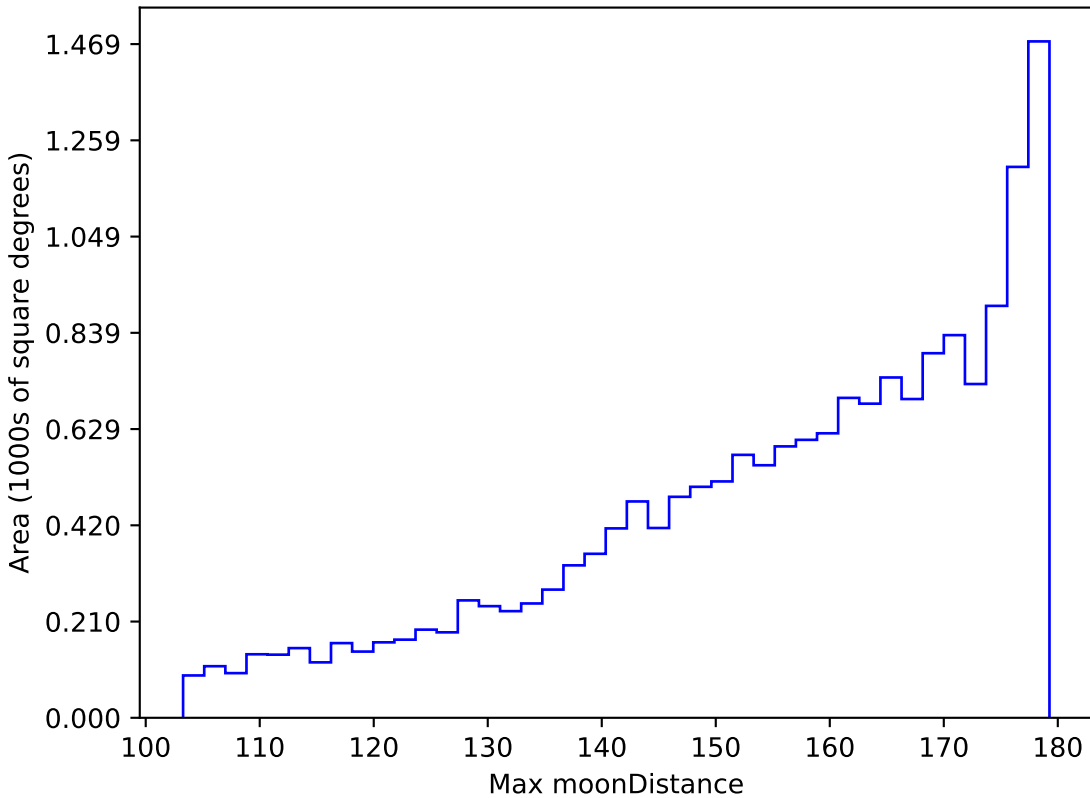
mw_roll_all_v3.3_10yrs WFD r band: Max moonDistance
