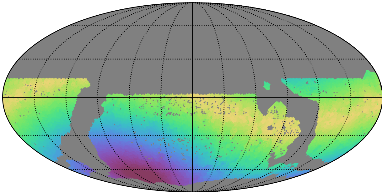
mw_roll_all_v3.3_10yrs WFD g band: Max moonDistance
