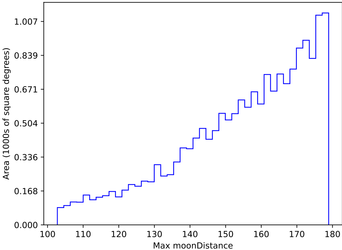
mw_roll_all_v3.3_10yrs WFD g band: Max moonDistance
