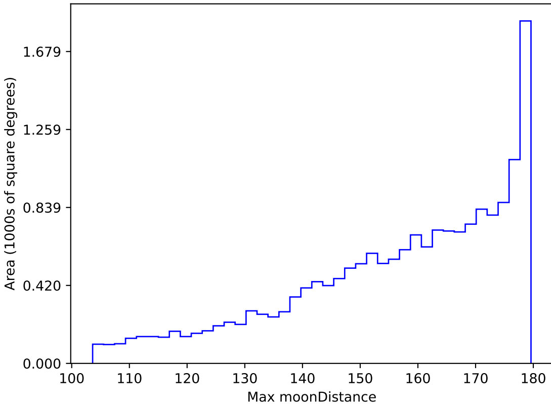
mw_roll_all_v3.3_10yrs WFD all bands: Max moonDistance
