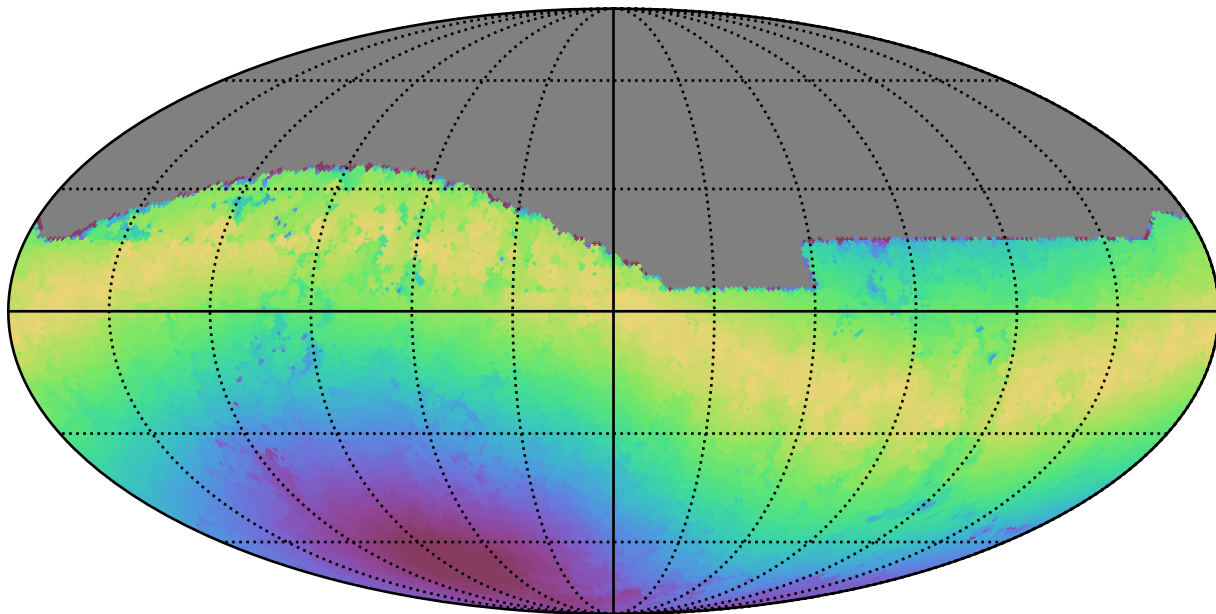
mw_roll_all_v3.3_10yrs All sky z band: Max moonDistance
